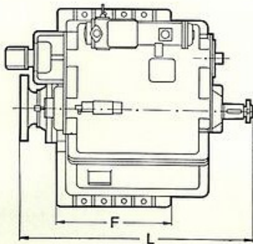
齿轮箱外形尺寸表 i=2:l 至 4:l Dimensionus for ratios from i=2:l up to 4:l only
